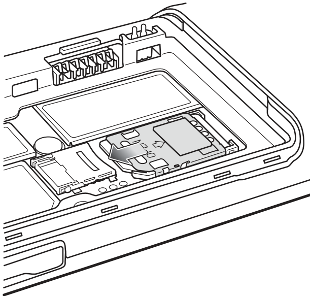
Figure 7: Lock SIM Card Holder
