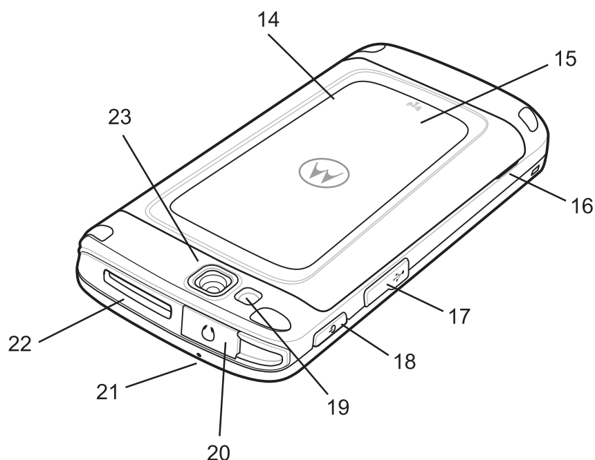
Figure 3: Back View
