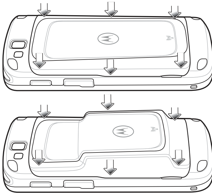
Figure 14: Secure Cover
