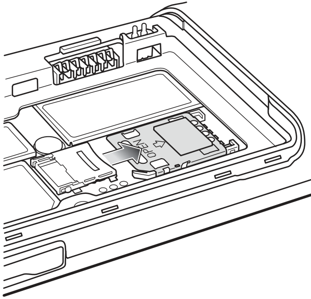
Figure 4: Unlock SIM Card Holder
