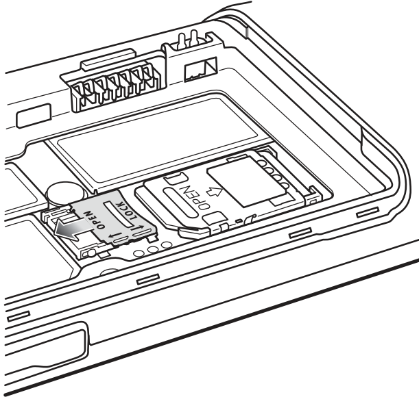
Figure 8: Unlock microSD Card Door
