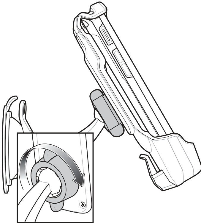
Figure 115: Tighten Nut
