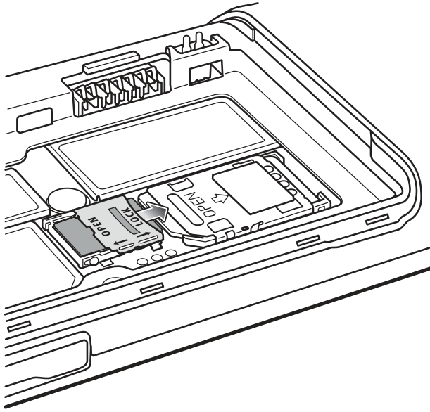
Figure 10: Lock SD Card Door
