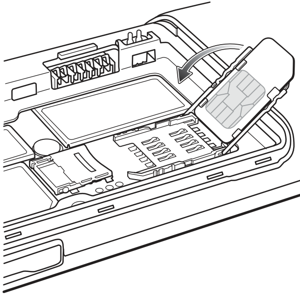
Figure 6: Close SIM Card Holder
