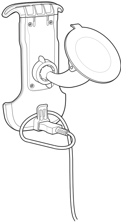
Figure 117: Cable Retention
