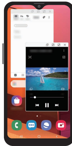
Pop-up view
