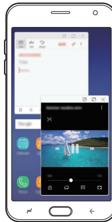
Pop-up view
