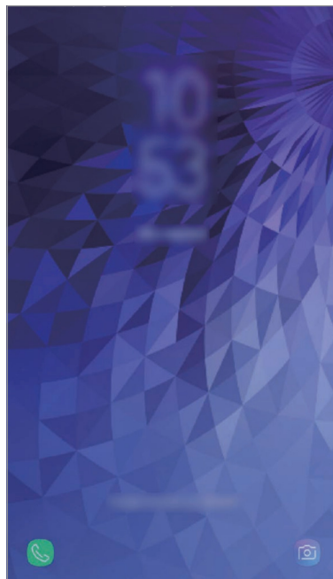
Locked screen
