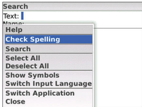
Figure 10. Full menu
