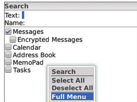
Figure 11. Short menu
