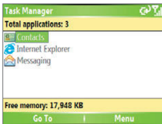
Task Manager
