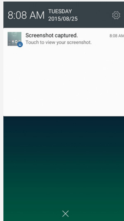
Figure 1: Notification
