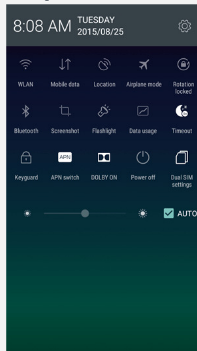
Figure 2: Quick Settings
