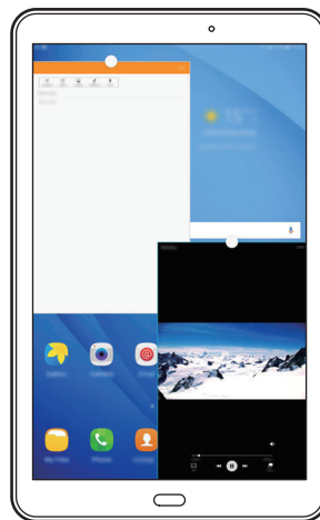
Pop-up view
