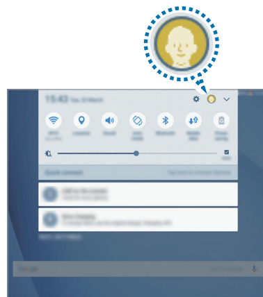
Notification panel
