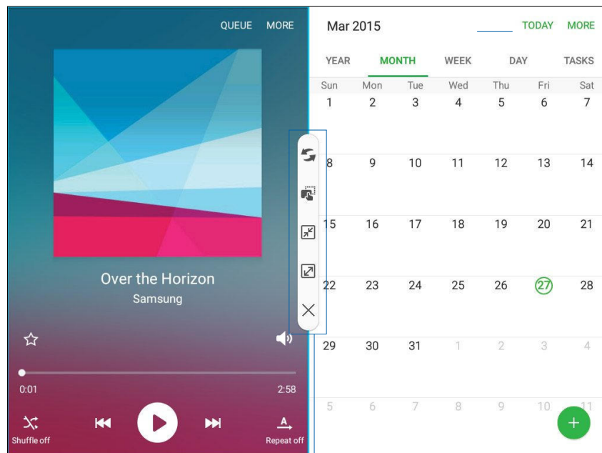
Window controls
